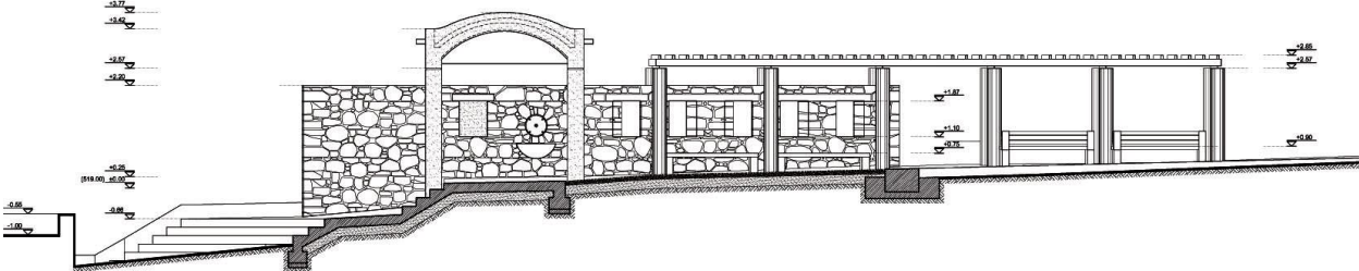
Arrangements in the square
