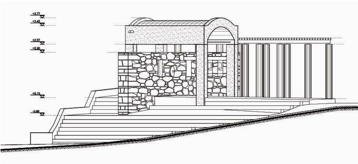
Arrangements in the square
