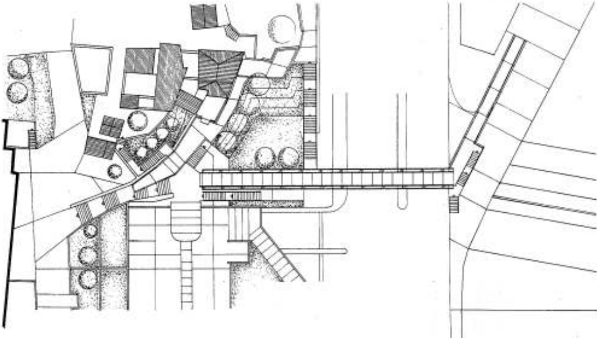
Pedestrians Overpass – Layout
